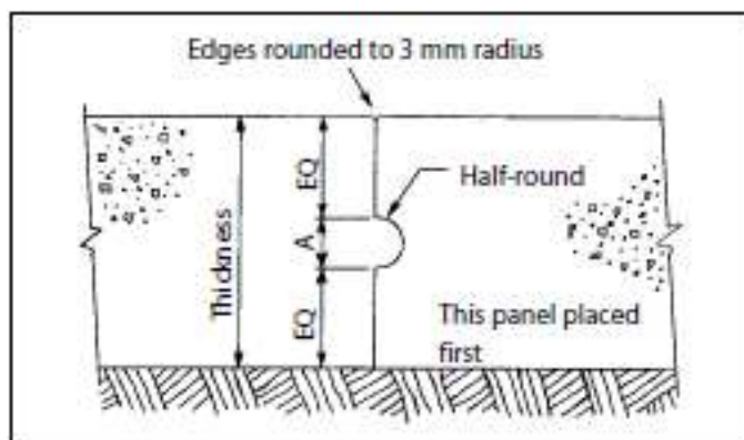
Figure 1: Construction joint
